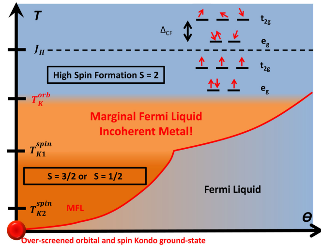
FIG. 1 (color online). Phase diagram of single Fe in an As tetrahedron. At T \sim J_H , the Hund’s coupling locks the spins of the Fe atom into an S = 2 state, and the orbital Kondo effect flows to strong coupling, giving rise to a marginal Fermi liquid overscreened state at T \sim T_K^{\text{orbital}} . The dangerously irrelevant spin-Kondo interaction finally drives the system to an overscreened spin-Kondo ground state at T_{K2}^{\text{spin}} . \theta is the deviation away from perfect tetrahedral symmetry, where \theta_c = 109.5^\circ , and will break the SU(2)^{\text{orb}} symmetry and restore Fermi liquid behavior.
