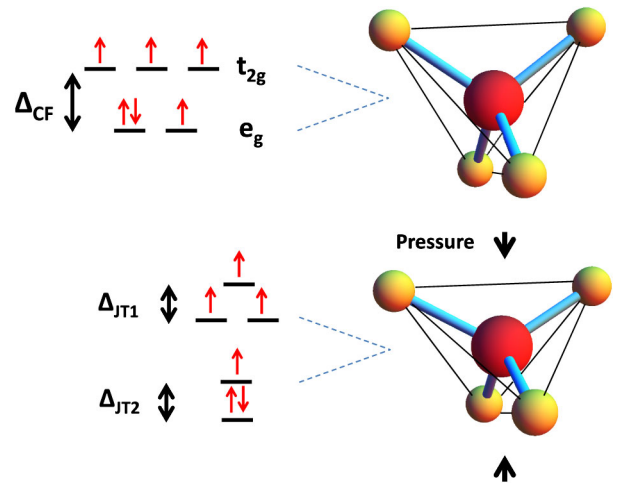
FIG. 2 (color online). Crystal field splitting of the d -electron orbitals in a tetrahedron into the upper t_{2g} and lower e_g orbitals. The lower diagram shows effect of compression along the c axis, which lifts the twofold degeneracy in the e_g orbitals.
