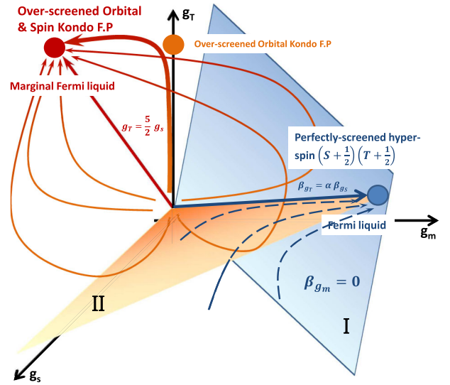
FIG. 4 (color online). Schematic plot of the RG flow. The perfectly screened hyperspin Fermi liquid fixed point lies along the line \beta_{g_T} = \alpha(S)g_S in plane I, and is stable against weak breaking of SU(4) symmetry [18]. For strong asymmetry, the system flows to the overscreened orbital and spin-Kondo marginal Fermi liquid fixed point. The blue plane I is defined by \beta_{g_m} = 0 , and the orange plane II is defined by \beta_{g_T} = \alpha(g_m, S)\beta_{g_S} . The bold line indicates the expected RG flow for a realistic FeAs tetrahedron.
