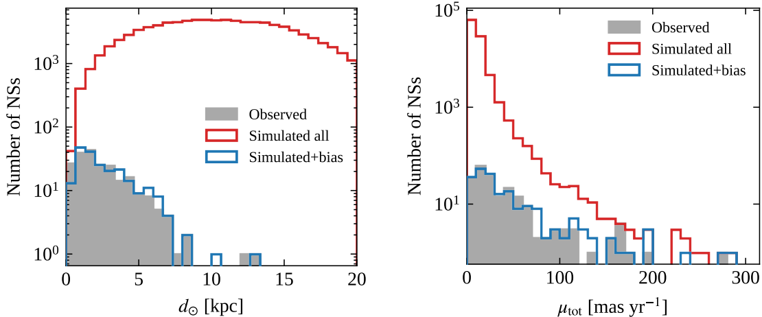
Figure 11. Distribution of heliocentric distances d_{\odot} (left panel) and proper-motion magnitudes \mu_{\text{tot}} (right panel) for the 216 neutron stars with measured proper motion (gray histograms). For comparison, we also show the distances and proper-motion magnitudes for 216 simulated neutron stars (blue histograms) randomly sampled from a mock population generated with the fiducial parameters \sigma_k = 265 \text{ km s}^{-1} and h_c = 0.18 \text{ kpc} (red histograms). For the weighted sampling, we use the weight function f(d_{\odot}) = d_{\odot}^{-1} \exp(-0.5d_{\odot}) .
