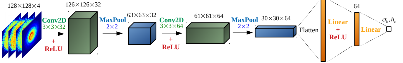
Figure 3. Schematic representation of our CNN architecture for an input of galactocentric maps with resolution 128 \times 128 and 4 channels (1 density map plus 3 velocity maps). A module formed by two blocks that each contain a convolution layer and max pooling layer is followed by a fully connected linear network with one hidden layer. The final network output is either a single parameter or two parameters depending on the experiment specifics.
