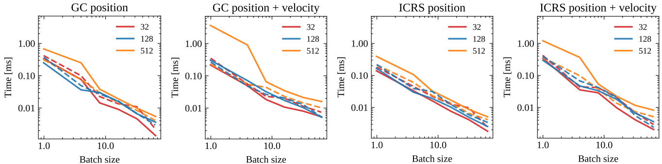
Figure 13. MLP forward ( solid lines ) and backward ( dashed lines ) pass times per sample in ms for the training process on the single parameter \sigma_k of the Maxwell kick-velocity distribution, as a function of the batch size and the resolution ( red, blue, and orange curves for 32, 128 and 512 respectively) using the four different input configurations T1 (GC position), T2 (GC position + velocity), T3 (ICRS position) and T4 (ICRS position + velocity).
