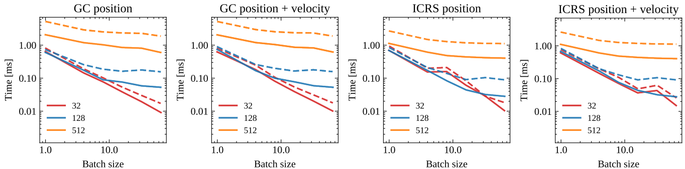
Figure 14. CNN forward ( solid lines ) and backward ( dashed lines ) pass times per sample in ms for the training process on the single parameter \sigma_k of the Maxwell kick-velocity distribution, as a function of the batch size and the resolution ( red, blue, and orange curves for 32, 128 and 512 respectively) using the four different input configurations T1 (GC position), T2 (GC position + velocity), T3 (ICRS position) and T4 (ICRS position + velocity).
