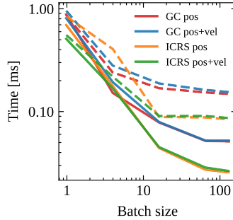
Figure 15. CNN forward pass ( solid line ) and backward pass time ( dashed line ) per sample for the two-parameter experiments as a function of the batch size for the four different input configurations T1 (GC position), T2 (GC position + velocity), T3 (ICRS position) and T4 (ICRS position + velocity).
