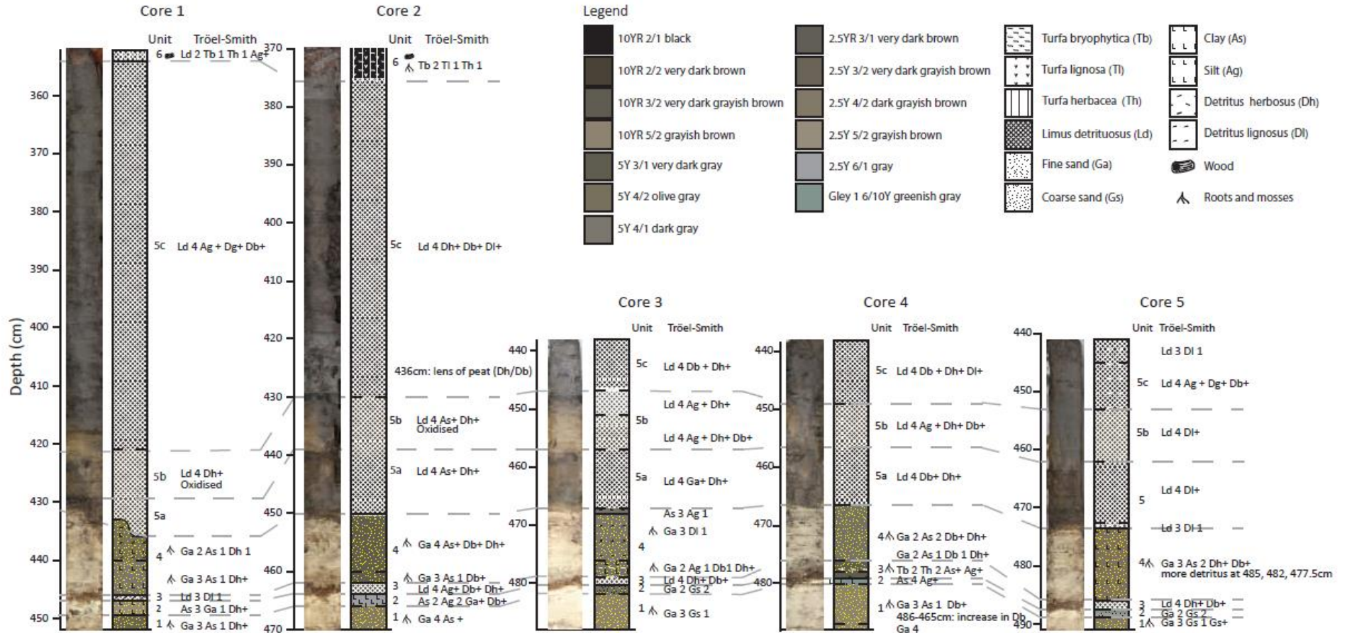
Appendix A.1. Images and descriptions of the lithostratigraphic units observed in five cores obtained from the Kingshouse 2 basal sedimentary sequence; note the clear consistency in the sequences of lithological units 1 to 5c and their boundaries.
