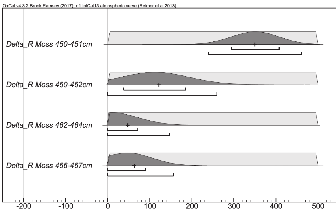
Figure 12. Potential reservoir effect (Delta R) of samples containing moss remains, derived from the age model constructions presented in Appendix A.6 .
