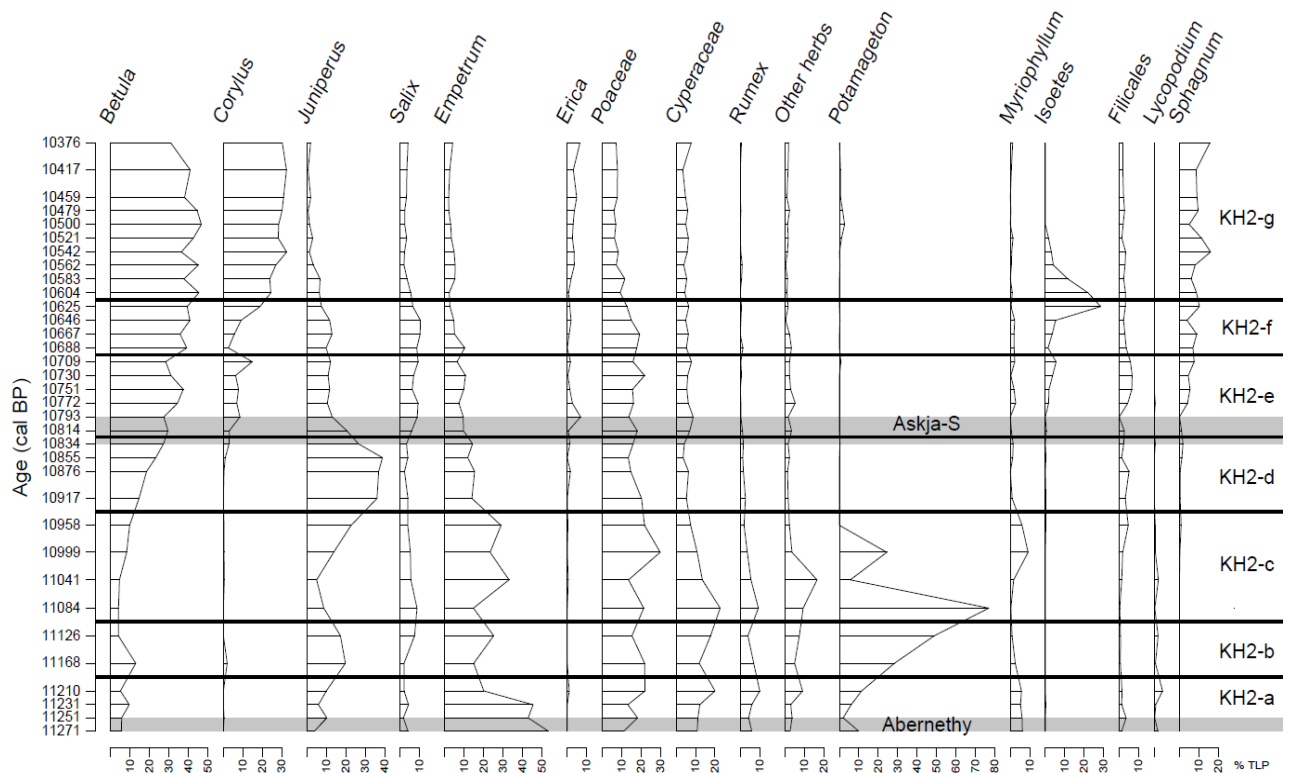
Figure 9. Percentage pollen data (% total land pollen) for selected taxa and the positions of the Askja-S and Abernethy tephras for the Kingshouse 2 sequence shown on a time axis using the Bayesian-based age model presented in Figure 8 and discussed in the text. The local pollen assemblages zones (final column) as in Figure 5 .
