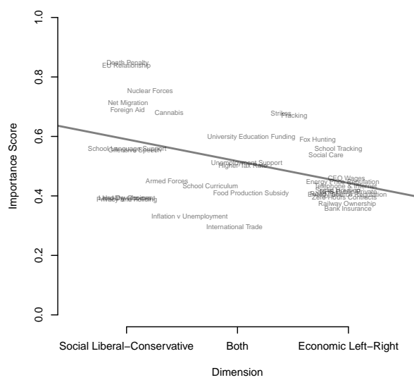
Figure 5: Top left: loadings of issues on economic left-right and social liberal-conservative dimensions. Top right: average 2D position of respondents by 2017 UK general election vote. Bottom: importance of each issue as a function of the extent to which it divides the public along the economic left-right versus the social liberal-conservative dimension.
