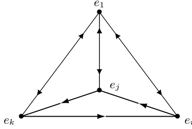
Fig. 1: Suspension trick: the cycle e_i \wedge e_j + e_j \wedge e_k + e_k \wedge e_i is equal to the boundary (e_1 \wedge e_i \wedge e_j)\delta_3 + (e_1 \wedge e_j \wedge e_k)\delta_3 + (e_1 \wedge e_k \wedge e_i)\delta_3 .
