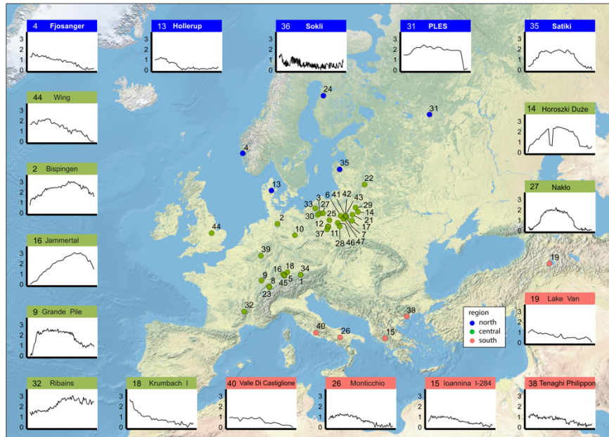
Figure 2. Map of the 47 analysed Eemian pollen sequences and individual sample scores (standard deviation units) of selected detrended canonical correspondence analysis (DCCA) axis 1 plots for 18 sequences (the remaining 29 sequences are in ESM 8). Colours of locations indicate assigned region (blue = north; green = central; salmon = south). The number at each location corresponds with sequence numbers in ESM 2. The sample scores are plotted with the oldest (bottom) at the far left and the youngest (top) at the far right. The individual sample scores are weighted averages of the response (pollen taxa) variable scores (also applies to ESM 8).
