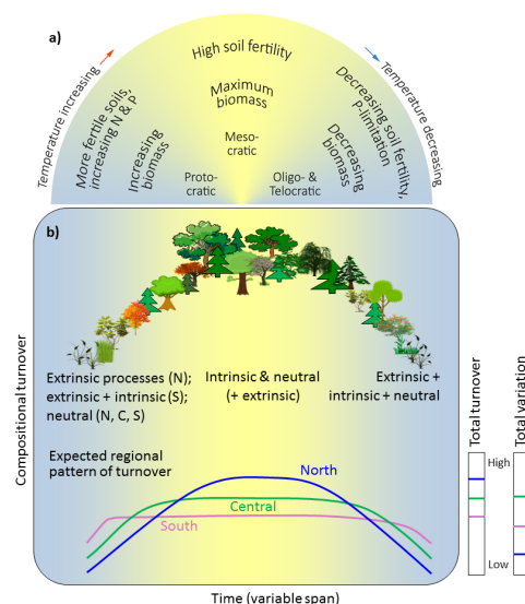
Figure 1. Hypothetical responses of an ecosystem in the last interglacial (Eemian) in terms of biomass and fertility (modified from Birks and Birks 2004). a) The three phases of Eemian vegetation history, namely protocratic, mesocratic, and oligocratic plus telocratic, in response to changing temperature (outer arc). b) Hypothetical model of compositional change (turnover) within an Eemian pollen sequence with expected patterns of turnover in each geographical region and an indication of total palynological turnover and total palynological variation expected in north (above 60°N), central (45–60°N), and south (below 45°N) Europe. The turnover axis can be, for example, an ordination axis.
