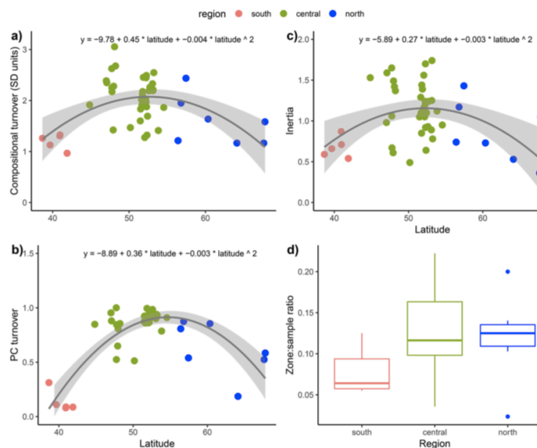
Figure 3 Total compositional turnover in each sequence plotted against latitude estimated by a detrended canonical correspondence analysis (DCCA; in standard deviation units) and b principal curves (PC; proportional distance); c total inertia or variation for each sequence estimated by DCCA; and d the proportions of optimal partitions to total number of samples in a sequence for each region. The fitted lines in a , b , and c are a fitted generalised linear model with a Gaussian distribution with a second-order polynomial (grey shading is the 95% confidence interval). The DCCA-based turnover for each sequence is estimated as the range in sample scores (weighted averages of the taxon scores) within the sequence.
