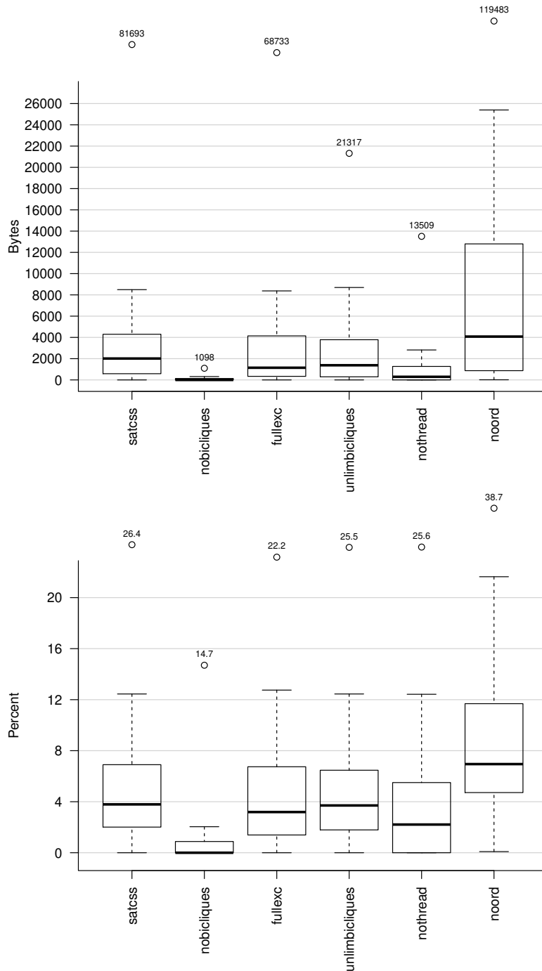
Figure 17: The savings in bytes (above) and in percentages (below) with certain optimisations disabled
