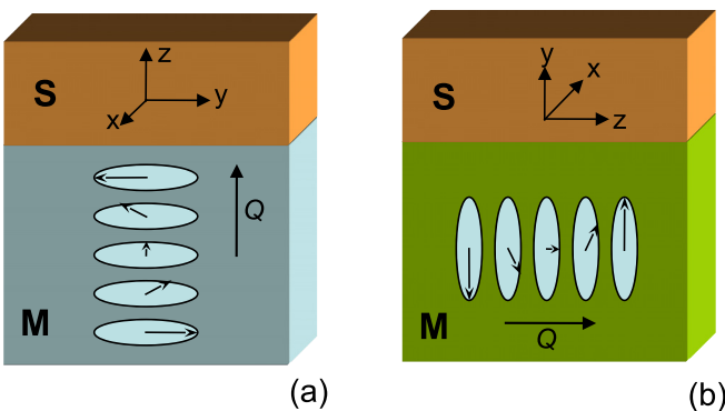
FIG. 1. The sketches of the spiral SSV in two configurations: spiral vector \mathbf{Q} (a) orthogonal to the superconducting interface (opening of the LRTC channel) or (b) parallel to the superconducting interface.
