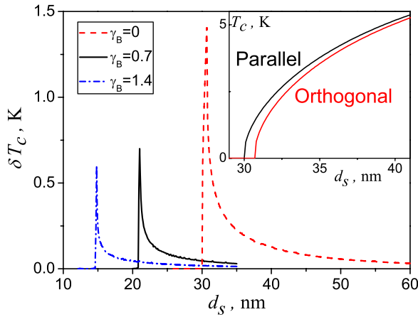
FIG. 2. Change in the superconducting critical temperature \delta T_c at the crossover between the two spiral configurations shown in Fig. 1 as a function of the S layer thickness d_s for different \gamma_b values.
