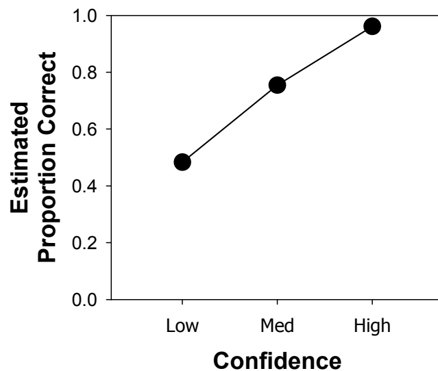
Figure 2. Estimated suspect ID accuracy (proportion correct) as a function of confidence for the data from the Houston Police Department field study (Wixted, Mickes, Clark, Dunn, & Wells, 2016).
