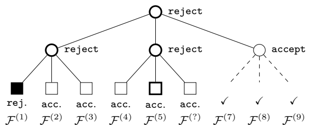
Figure 1: Traversing the file tree spanned over nine different outsourced files. Four times CSPoRP is performed ( \circ ) and six times PoRec ( \square ). As a result \mathcal{F}^{(1)} is damaged beyond repair ( \blacksquare ), \mathcal{F}^{(5)} is damaged but recoverable ( \square ), and all other files are sound and recoverable.
