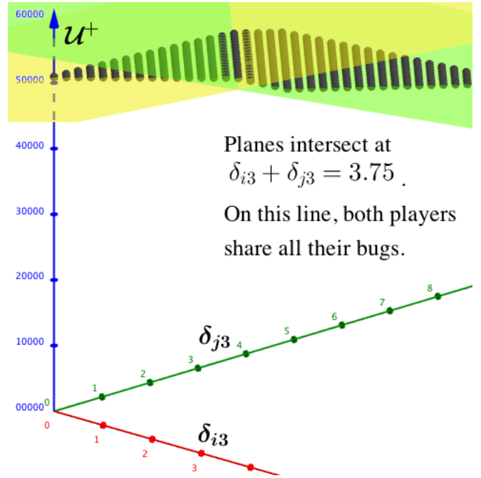
Figure 2: A 3D plot of U^+ as a function of (\delta_{i3}, \delta_{j3}) . All other parameters as in Table 1. The plot shows that the mutual value of a fair trade is maximised when players have a balanced view on the competitive value of each bit of information.
