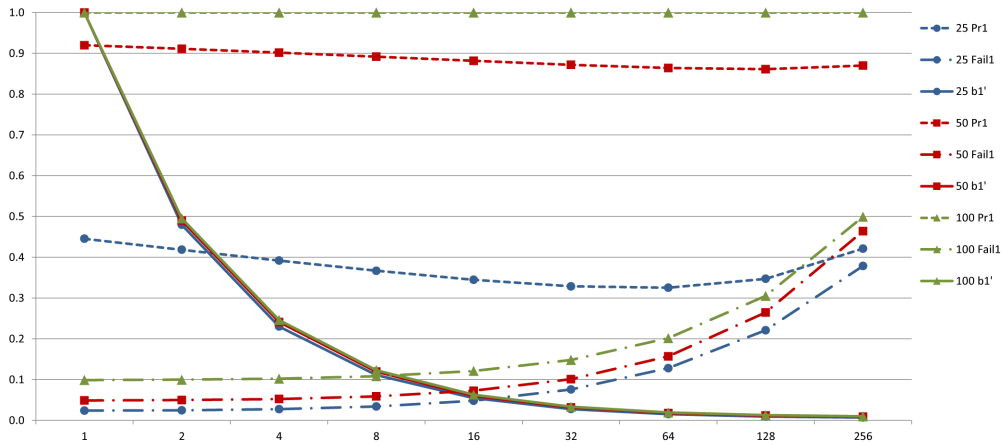
Figure 4: Plot of the values of \text{Pr}_1 , \text{fail}_1 and b'_1 when \mu = 1 and there are 1, 2, 2^2, \dots, 2^8 nodes per tree for key storage \sigma = 25, 50 and 100 respectively
