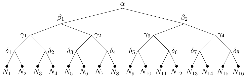
Figure 2: LKH tree on 16 nodes
