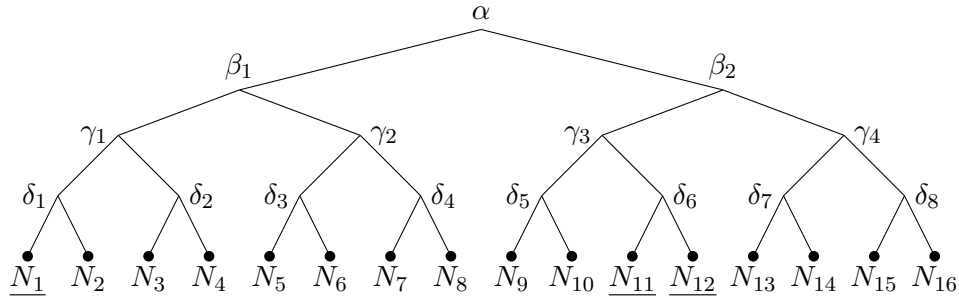
Figure 6: LKH tree on 16 nodes
