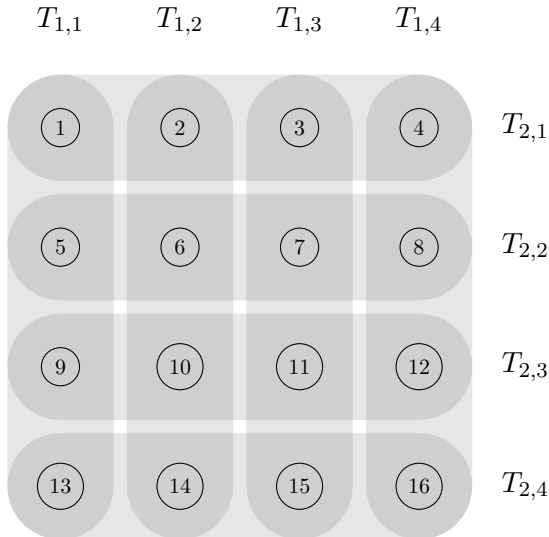
Figure 3: Example of partitioning nodes into L = \frac{\mu v}{\lambda} trees
