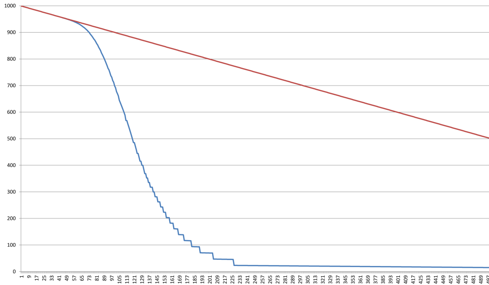
Figure 1: Plot of the deterioration of v(i) (Equation (18)) in comparison to the straight line (v - i) for an example network of v = 1000 nodes, where n = 1000 and k = 30 .
