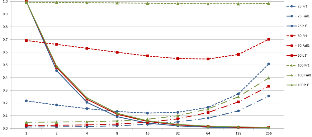
Figure 5: Plot of the values of \text{Pr}_1 , \text{fail}_1 and b'_1 when \mu = 2 and there are 1, 2, 2^2, \dots, 2^8 nodes per tree for key storage \sigma = 25, 50 and 100 respectively
