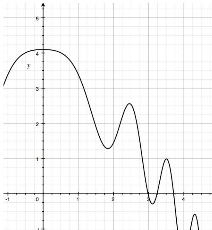
Figure 3: A representation in the two-dimensional Cartesian plane of a curve, f(x) .
