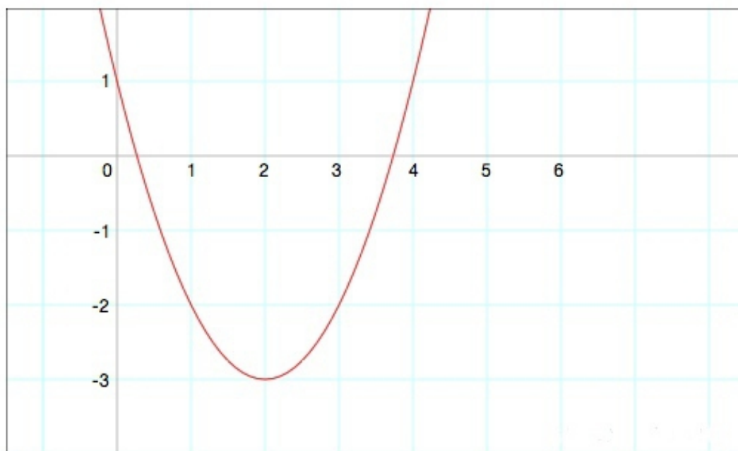
Figure 6: A representation in the two-dimensional Cartesian plane of the equation y = x^2 - 4x + 1 .
