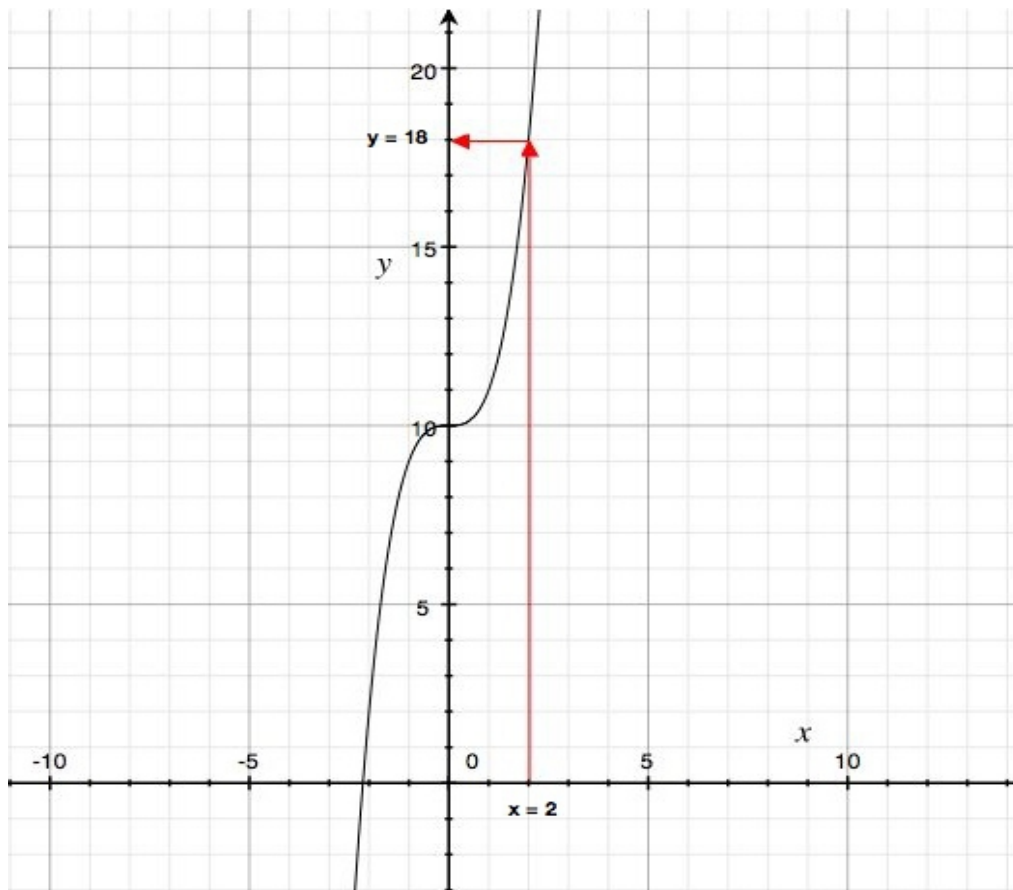
Figure 1: A geometric representation in the two-dimensional Cartesian plane of the complex polynomial y = x^3 - 4i^2 + 6 . As indicated, where x = 2 , y = 18 .
