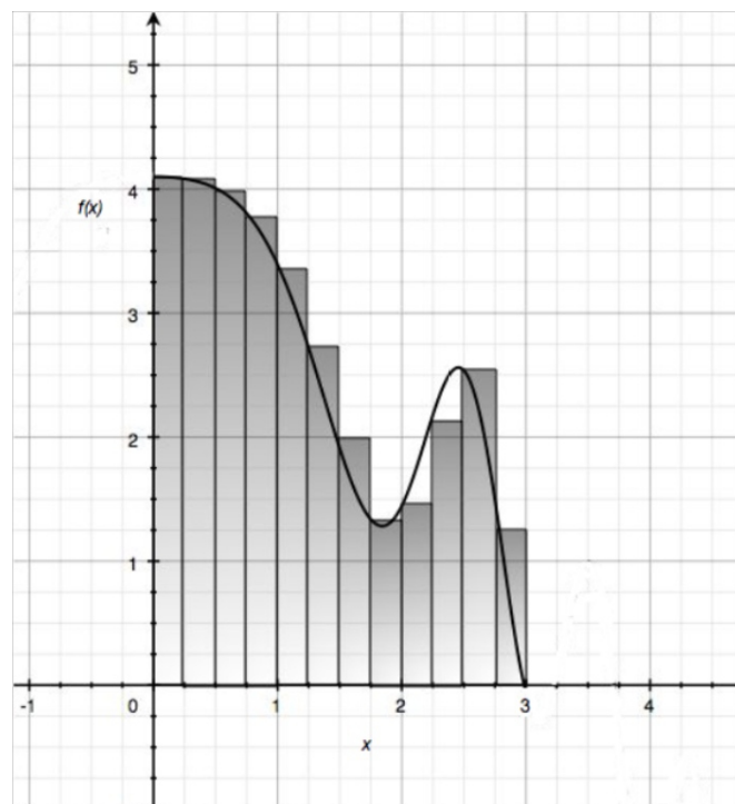
Figure 4: A representation of the curve f(x) . The rectangular sections approximate the area under the curve, where 0 \leq x \leq 3 and y \geq 0 , and are marked at intervals of width 0.25.
