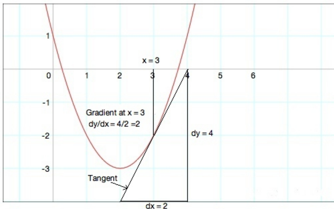
Figure 8: A representation of y = x^2 - 4x + 1 , with a tangent drawn at x = 3 .
