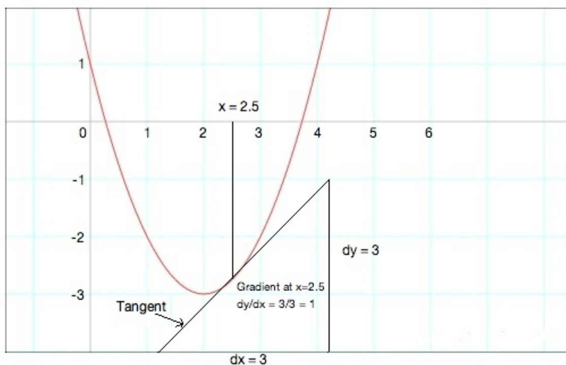
Figure 7: A representation of y = x^2 - 4x + 1 , with a tangent drawn at x = 2.5 .
