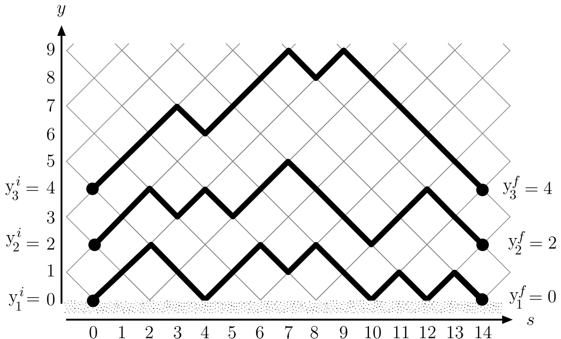
Figure 1: Three non-intersecting directed walks of length t = 14 in a watermelon configuration tied to the surface, where y_j^i = y_j^f = 2(j - 1) . The coordinates for the rows y and columns s are shown. Also illustrated are the positions of the walks in the columns s = 0 and s = t which are denoted by y^i and y^f respectively. The walk closest to the lower wall has weight \kappa^5 .
