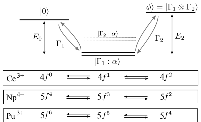
FIG. 2. Virtual charge fluctuations of a two channel Anderson impurity, where the addition and removal of an f -electron occur in channels \Gamma_1 and \Gamma_2 of different crystal field symmetry. The ground state is a Kramer's doublet, while the excited states |0\rangle , |2\rangle are singlets. The excited doublet |\Gamma_2 : \alpha\rangle represents a higher lying crystal-field level and is excluded from the Hilbert space of the problem. The relevant charge states of \text{Ce}^{3+} ( 4f^1 ), \text{Np}^{4+} ( 5f^3 ) and \text{Pu}^{3+} ( 5f^5 ) are indicated.
