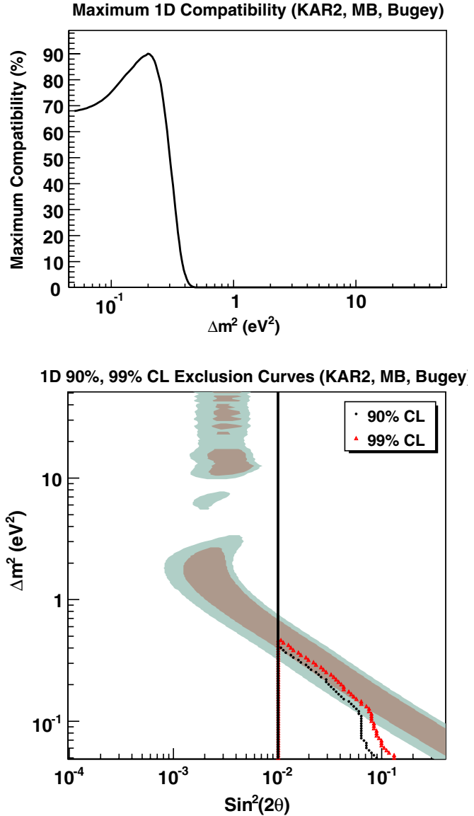
FIG. 9 (color online). Top: Maximum compatibility as a function of \Delta m^2 for the 1D KARMEN2, MiniBooNE, and Bugey analysis. Bottom: Exclusion bands (90%, 99%) found for the 1D KARMEN2, MiniBooNE, and Bugey joint analysis. Values to the right of the lines are excluded at the 90%, 99% CL. Triangle points form the 99% CL band, circle points form the 90% CL band. The vertical straight edge on the left indicates the lower \text{sin}^2 2\theta bound of 0.01.
