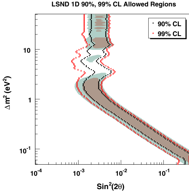
FIG. 3 (color online). 90% and 99% allowed regions for the 1D scan of LSND, overlaid on the 2D published allowed regions. Triangle points contain the 99% CL region, circle points contain the 90% CL region.
