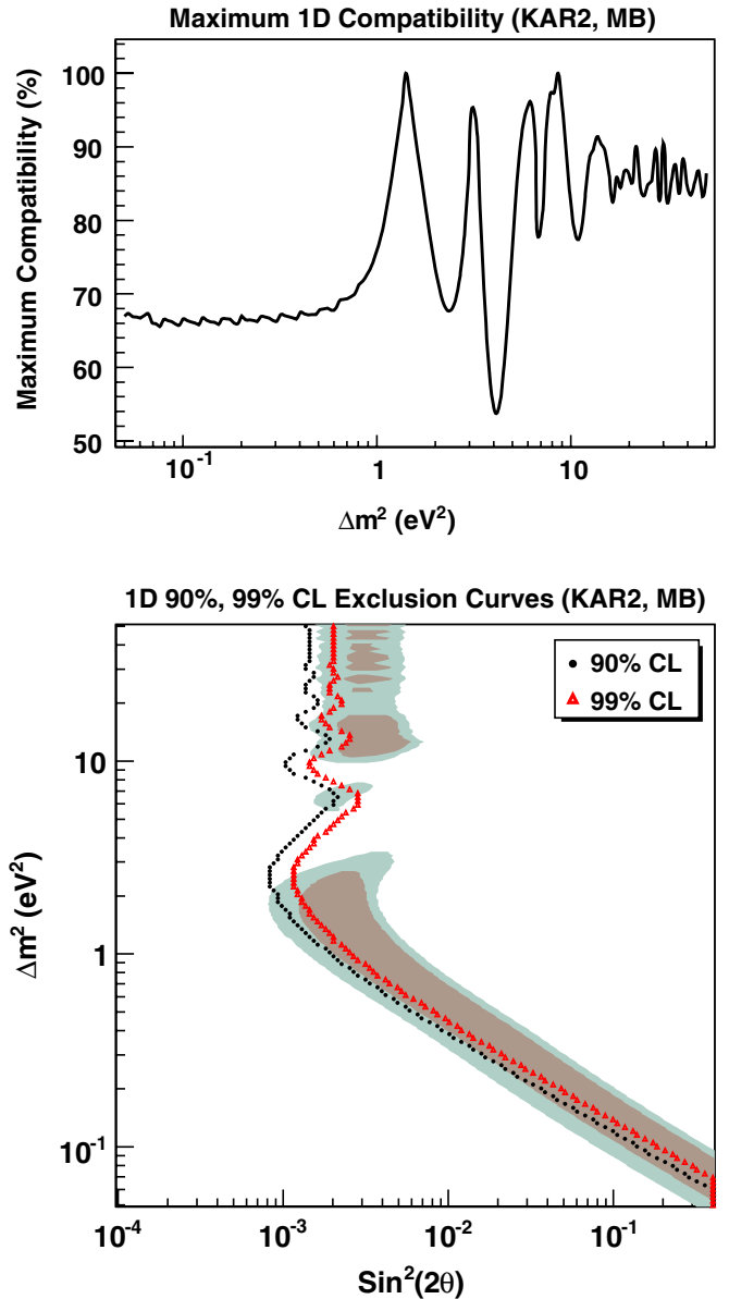
FIG. 7 (color online). Top: Maximum compatibility as a function of \Delta m^2 for the 1D KARMEN2 and MiniBooNE analysis. Bottom: Exclusion bands (90%, 99%) found for the 1D KARMEN2, and MiniBooNE joint analysis. Values to the right of the lines are excluded at the 90%, 99% CL. Triangle points form the 99% CL band, circle points form the 90% CL band. These curves are very similar to those found using the 2D method in Fig. 6.
