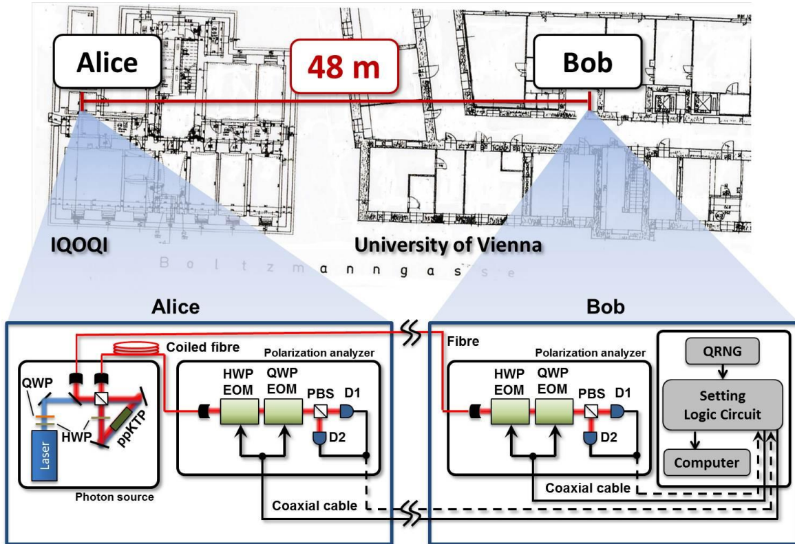
Figure 2: Experimental setup. The loophole-free steering experiment was carried out between two buildings: the University of Vienna and the Austrian Academy of Sciences (IQOQI). A polarization-entangled photon pair is generated by Alice using an entangled photon source 20,21 . For each entangled pair, one photon is kept in an 80 m long, coiled optical single-mode fibre (red line) on Alice's side, located next to the source. The other photon is sent to Bob via another optical fibre. On Bob's side, one of three measurement settings is chosen by his fast home-made quantum random number generators (QRNG) based on [22] and sent to Alice's side via the classical link. The setting choice is stored locally and also sent to Alice via a low-dispersion coaxial link and subsequently applied to both photons (solid black lines). Alice's polarization analyzer implements the different settings with two electro-optical modulators (EOMs) realizing ultra-fast switchable half- and quarter-wave plates (HWP, QWP), as well as a polarizing beam splitter (PBS) and two home-made photon detector modules based on silicon avalanche photo-diodes ( D_i ). On Bob's side there is an equivalent polarization analyzer. The results are then collected (dashed black lines) in Bob's lab and compared in a logic circuit.
