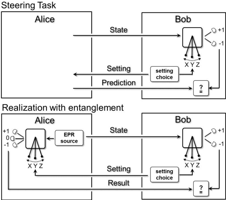
Figure 1: Top: In a steering experiment, Alice sends a system to Bob that he assumes to be an unknown local quantum state 5-7 . Next Bob chooses freely in which setting (X, Y or Z) to measure. Then he sends his choice of setting to Alice and records secretly his measurement result. Bob now challenges Alice, who claims that she can steer his state from a distance, to predict his result (+1, -1). Provided the correlation between her prediction and his result is above the steering bound, Bob is forced to conclude Alice indeed remotely steered his state (spooky action at a distance), or give up his assumption of a local quantum state. Bottom: Using entangled pairs of photons produced by an EPR source Alice can demonstrate steering. She measures
