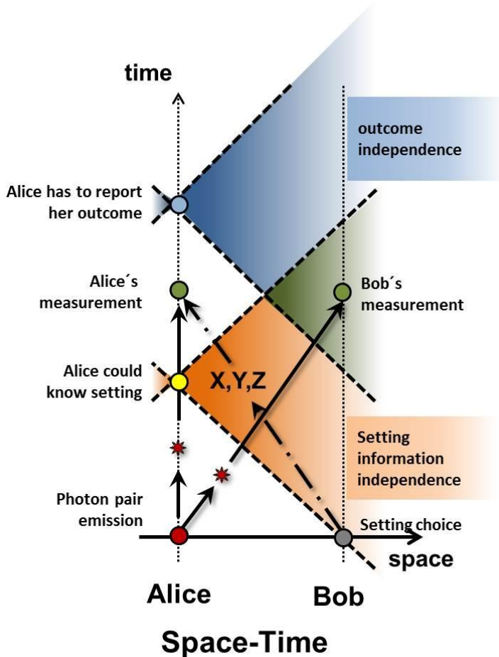
Figure 3: Space-time diagram illustrating the conditions to close the locality and freedom-of-choice loopholes (illustration, not to scale): Firstly, Alice creates a photon pair and sends a photon to Bob before she receives Bob's setting choice. In our experiment, we enforce freedom of choice by space-like separating the generation of the entangled photon pairs (red dot), and the QRNG's choice (grey dot). They happen 48 m apart at the same time ( t=0 ) in the lab frame. The second condition is to exclude any causal influence of Alice on Bob's measurement once she can know the setting. This setting information independence is enforced in our experiment by Bob's measurement taking place in a region (orange area) that is space-like separated from the event (yellow dot) marking the time at which Alice could in principle know Bob's setting. Lastly, we also ensure that Alice cannot know Bob's measurement outcome before reporting hers, since reproducing any arbitrary correlation would then become a trivial task for her. This outcome independence is guaranteed by the event of Alice's outcome report (blue dot) being space-like separated (blue area) from Bob's measurement event (left green dot).
