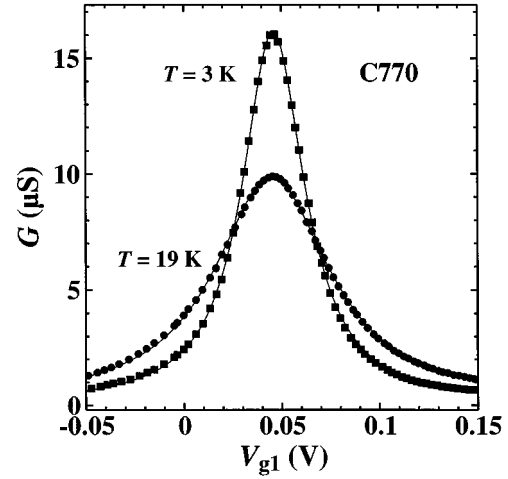
FIG. 2. Equilibrium tunneling conductance G(V_{SD}=0) as a function of the gate voltage V_{g1} controlling the carrier density in the upper layer, when the lower layer density is fixed at n_2 = 3.25 \times 10^{11} \text{ cm}^{-2} . The traces were taken at T = 3 K (squares) and 19 K (circles), and the solid lines are the fits to Eq. (10).
