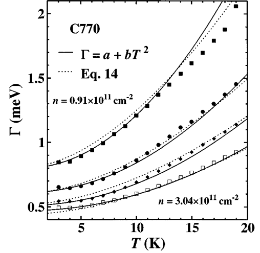
FIG. 4. Temperature dependence of the equilibrium linewidth \Gamma for n_1=n_2=0.91, 1.62, 2.19, 3.04\times 10^{11}\text{ cm}^{-2} . The solid lines are fits to the form a+bT^2 , and the dashed lines are obtained from the best fit to Eq. (14).
