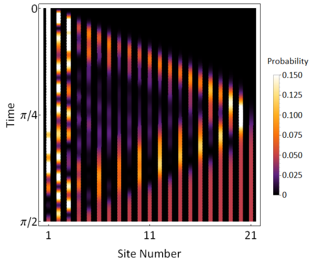
FIG. 1: Time evolution of probability of excitation being at each site in a 21 qubit chain, approximating the evolution of |1\rangle evolving to the W -state.
