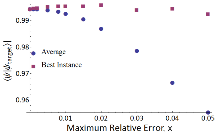
FIG. 2: Overlap of output with target W state in a chain of 99 spins, comparing average over 400 instances with the best sample, where each magnetic field and coupling strength is altered by multiplication of an amount chosen uniformly at random from the range 1 \pm x .
