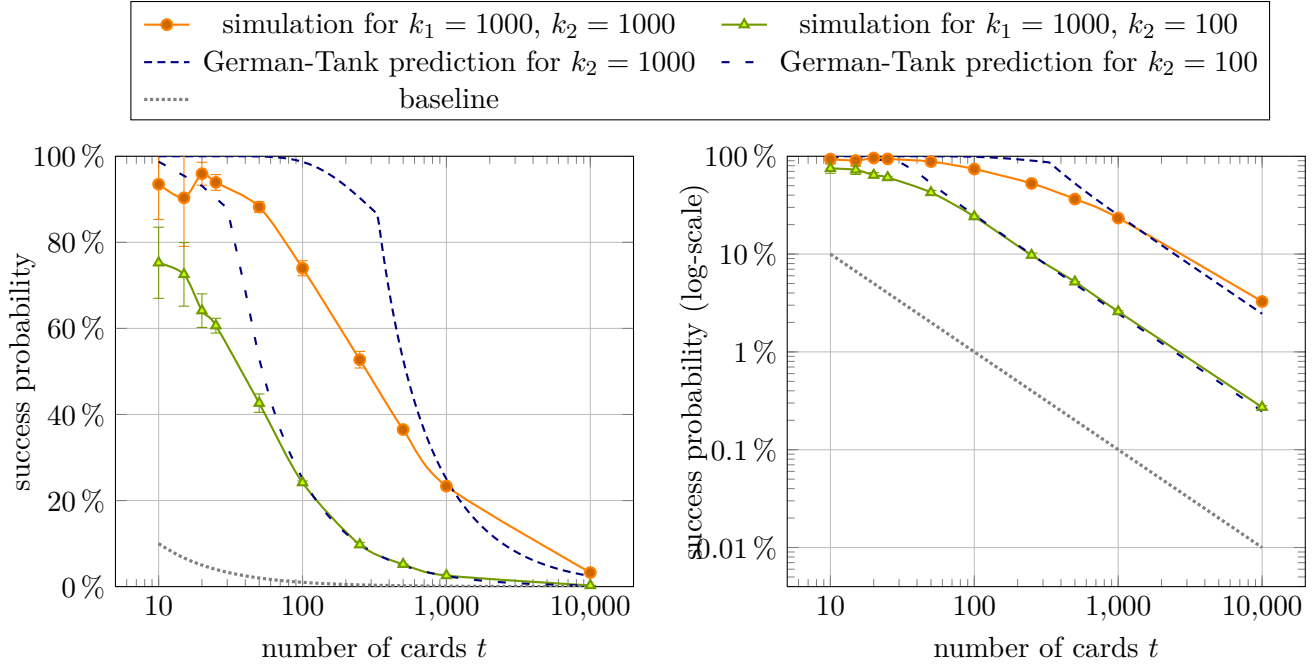
Figure 3: Results of the statistical analysis for the basic skill-key fingerprinting scenario: the predicted success probability of the attack refers to k_1 = 1000, k_2 = 100 (loosely dashed) and k_2 = 1000 (densely dashed). The baseline indicates the success probability of an adversary that tries to win the game by pure guessing. The number of cards t on both sides and the success probability on the right side are displayed in logarithmic scale; error bars show the standard deviation.
