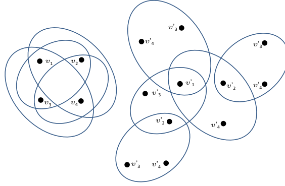
Fig. 2. The instance I described in Example 3 and the corresponding instance I_B^{ord}
