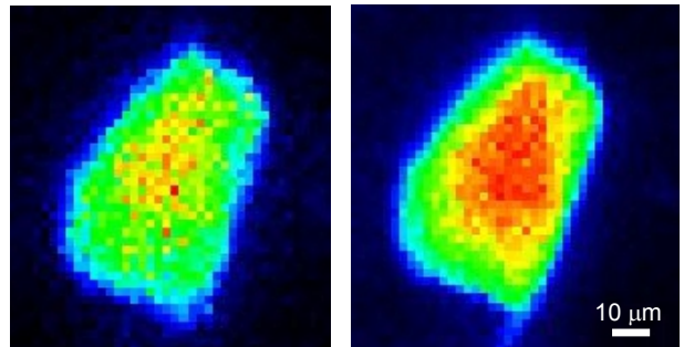
FIG. 1: Elemental distribution of Ti (left) and Zn (right) in the recovered sample. Variations in the fluorescence intensity are due to variations in the sample thickness.
