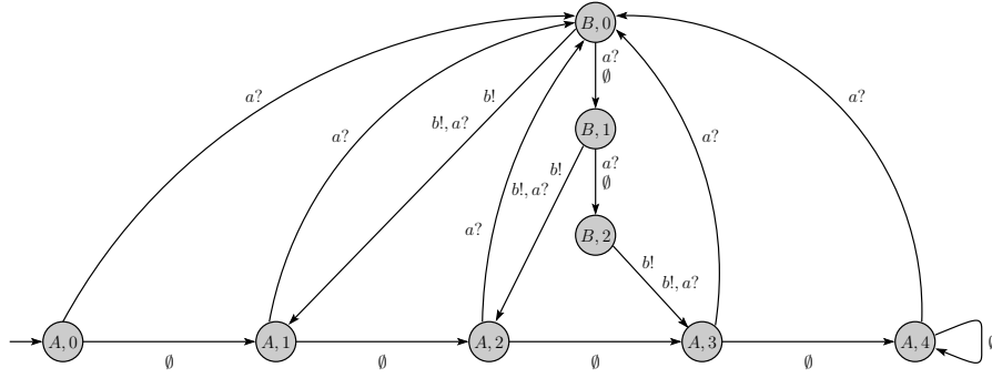
Fig. 5. Büchi automaton \mathcal{B}_{\mathcal{M}^x} corresponding to DTIOM \mathcal{M}^x (unreachable states have been removed)
