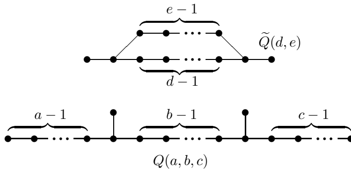
Figure 6. The graphs \widetilde{Q}(d, e) and Q(a, b, c) .
