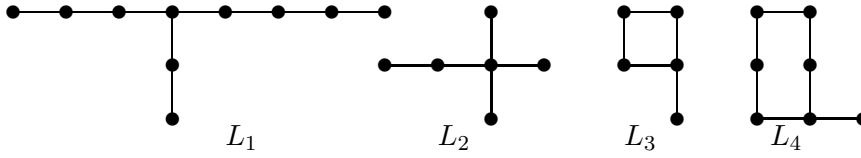
Figure 4. The graphs L_1, \dots, L_4 .
