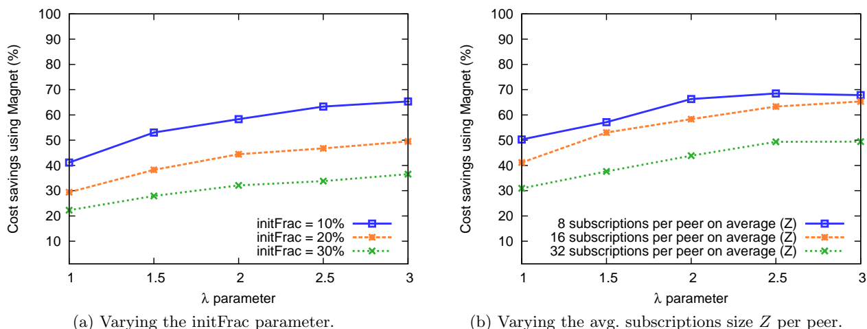
Figure 8: HIERARCHICAL-TOPICS model: MAGNET’s performance improves with increased subscription correlation (higher value of \lambda ). Higher values of \text{initFrac} imply fewer exploitable correlations, supporting the trend seen on the curve on the left. Increasing the average degree Z while keeping \text{initFrac} constant incorporates randomness from the initialization stage as suggested by the decline on the right. We see that MAGNET brings significant cost savings over the strawman approach on the HIERARCHICAL-TOPICS model.
