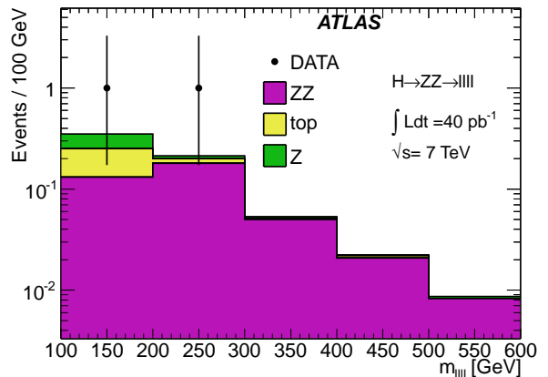
Fig. 5. Distribution of m_{\ell\ell\ell\ell} in the H \rightarrow ZZ^{(*)} \rightarrow \ell\ell\ell\ell search before applying the lepton impact parameter and isolation requirements which remove the two candidates. The error bars reflect Poisson asymmetric errors.
