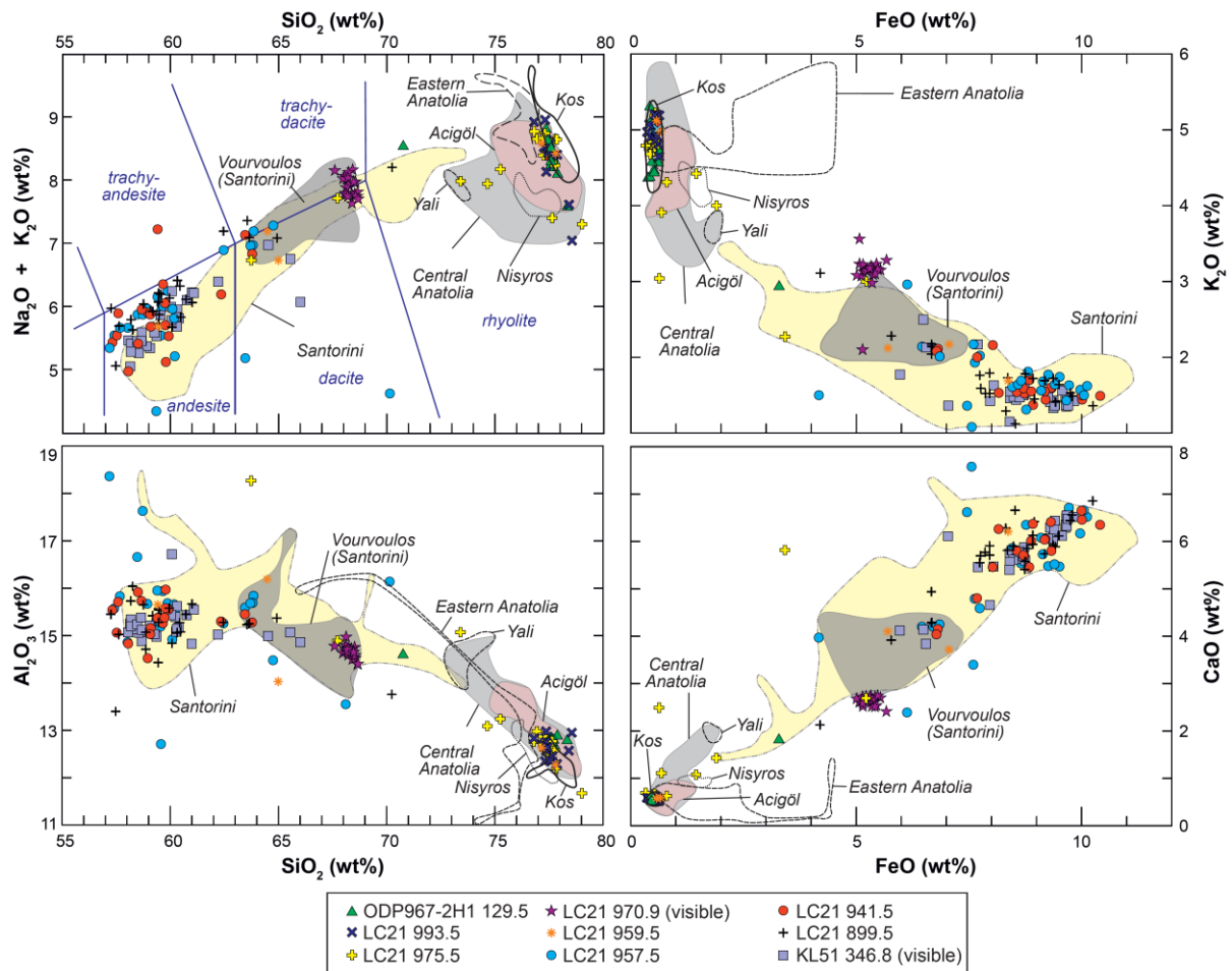
Figure 5. Top left: Total Alkali vs. Silica (TAS) diagram (after [77]) showing samples analysed in this study. Other panels show selected major element biplots of glass geochemistry from Electron Probe Microanalysis (EPMA) of the tephra samples in this study. Reproducibility is <10% relative standard deviation for analytes with concentrations >0.8 wt% with the exception of Na 2 O (14-15%). Full analytical results and standard analyses are provided in the supplementary data. Data for the LC21 970.9 (visible) tephra and LC21 957.5 are from [17]. Also shown are analyses of proximal tephras for comparison from: Santorini [48], Eastern Anatolia [78]; Central Anatolia including Acigöl [48,79]; Kos [17]; Nisyros [58]; Yali [13-14]. The geochemical field defined by proximal analyses of the Vourvoulos eruption of Santorini is shown separately from the rest of the Santorini field; see discussion in text.
