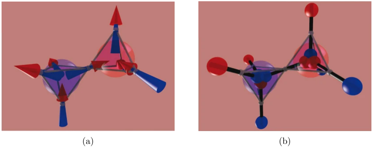
Figure 1.14: Representation of a thermal excitation in a classical spin ice in (a) the dipole representation by flipping a shared spin, and (b) the “Dumbbell” model by swapping two charges of opposite sign. Figures acquired from [105].
