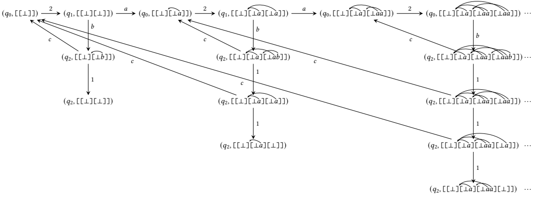
Fig. 5. The edge labelled graph generated from the CPDA with input from Example 8.2.
