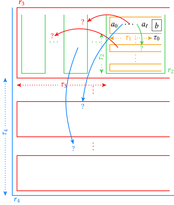
Fig. 2. Illustration for the proof of Theorem 2.8 when n = 4 . Missing states (?) in k -link's target are retrieve by reading top_{k+1}(s) from r_k . For every k , \tau_k^+ is obtained by composing the \tau_i s for i \leq k .
