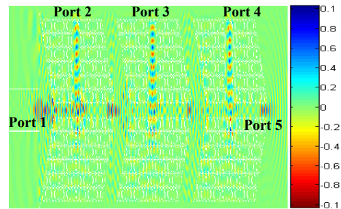
Fig. 4b Snapshot of the electric field when the control beam is ON and d = 8s (the ports 2, 3 and 4 are ON)
