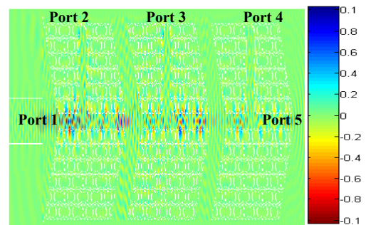
Fig.7. Snapshot of the electric field when the control beam is OFF (the ports 2, 3 and 4 are off) and d = 8a
