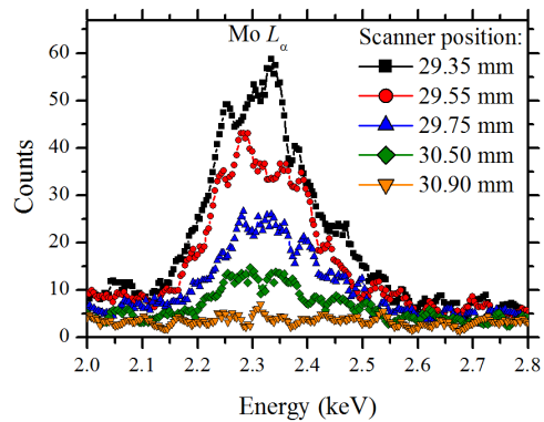
Figure 6. Molybdenum X-ray spectrum change during scanning
