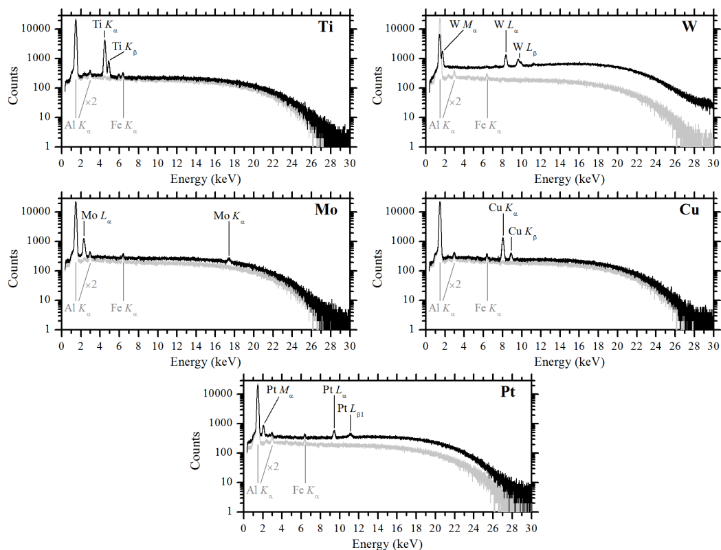
Figure 4. X-ray spectra of the wires (black line) and background (gray line).
