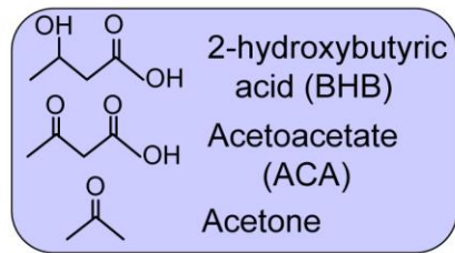
Ketone bodies
