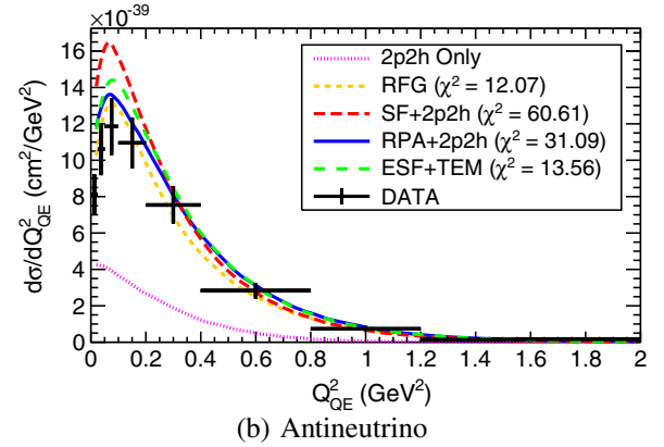
FIG. 6. Nominal model predictions for the MINERνA datasets with M_A = 1.01 \text{ GeV}/c^2 and all other model parameters at their default values. The relativistic RPA model is shown.
