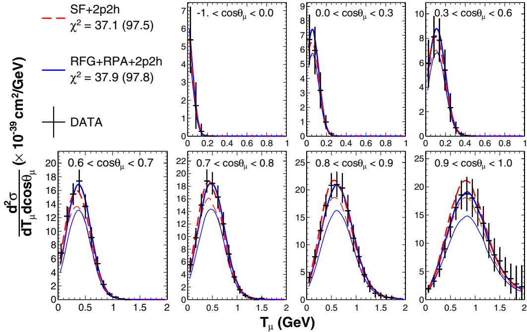
(a) Neutrino
