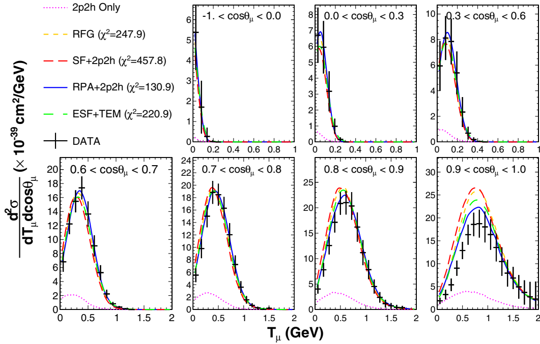
(a) Neutrino
