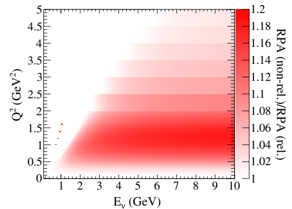
(b) \bar{\nu}_\mu - {}^{12}\text{C}
