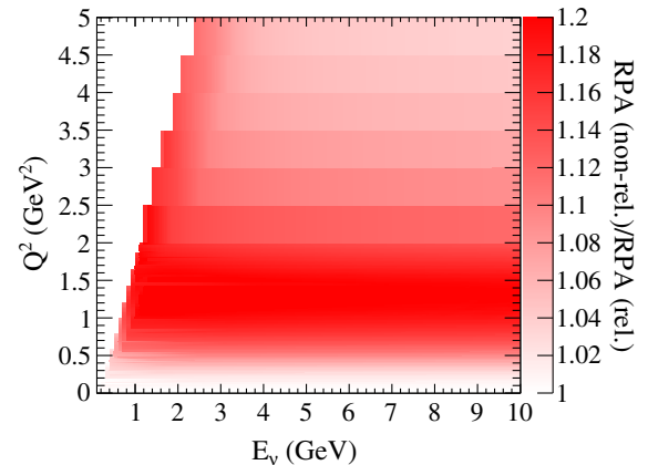
(a) \nu_\mu - {}^{12}\text{C}
