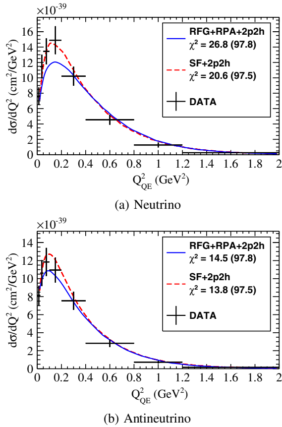
FIG. 10. Comparison of the best fit from the combined fits detailed in Table IV with the MINER \nu A datasets used in the fit. The \chi^2 values in the legend are the contribution from each dataset at the best-fit point (and the total \chi^2_{\min} for the combined fit).
