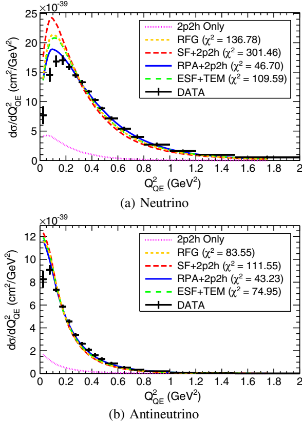
FIG. 7. Nominal model predictions for the MiniBooNE single-differential datasets with M_\Lambda = 1.01 \text{ GeV}/c^2 and all other model parameters at their default values. The relativistic RPA calculation is shown. Normalization parameters are applied as given in Table III.
