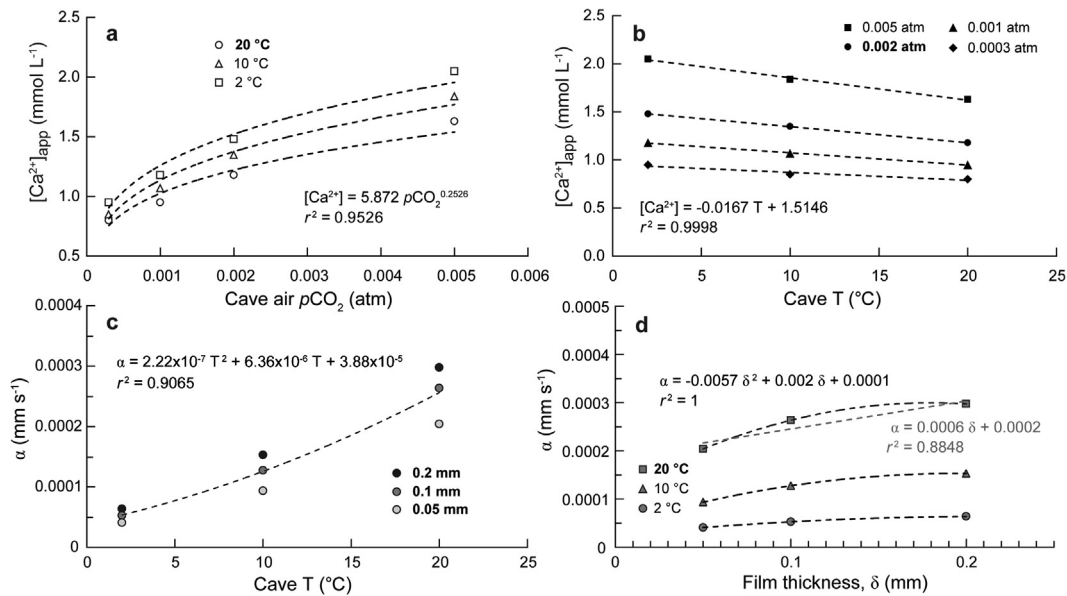
Fig. 2. A synthesis of data originally presented by Dreybrodt (1999) and transfer functions derived from these data by bivariate regression, which are used in the time series growth reconstruction for Gib04a. (a) A power law fit (correlation coefficient, r^2 = 0.95 ) between [Ca^{2+}]_{app} and cave atmosphere pCO_2 for a constant cave temperature of 20 °C. (b) A linear fit ( r^2 = 0.99 ) between [Ca^{2+}]_{app} and temperature for a constant pCO_2 of 0.002 atm. (c) A 2nd-order polynomial fit ( r^2 = 0.91 ) between the 'kinetic constant' ( \alpha ) and cave temperature for all data. (d) A 2nd-order polynomial fit ( r^2 = 1 ) between \alpha and film thickness ( \delta ) for a constant temperature of 20 °C. A linear fit ( r^2 = 0.89 ) is also shown for comparison, but not used in the growth reconstruction (grey line). Terms are defined in the text.
