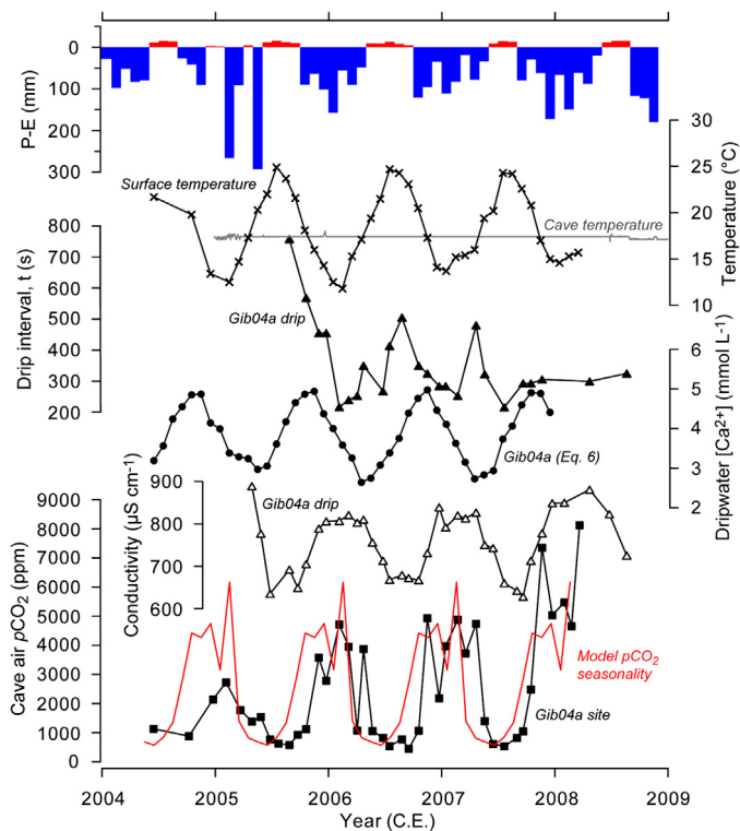
Fig. 3. Monitoring data (2004–2009) from the Gib04a drip site in NSM Cave (Fig. 1) and calculated model parameters: cave atmosphere p\text{CO}_2 spot measurements (squares) and monthly mean trend (red line); dripwater electrical conductivity (triangles); modelled dripwater [\text{Ca}^{2+}] using Eq. (6) (circles); drip discharge (filled triangles); surface temperature measured at Gibraltar's RAFMO station (crosses) and continuously logged cave air temperature (grey line); surface water excess (blue – positive, red – negative) calculated by subtracting potential evapotranspiration ( E ) from total monthly rainfall (GNIP data). We calculated E according to the method of Thornthwaite (1948), following Matthey et al. (2008), with heat index values and reduction factors taken from Patra (2001). Cave monitoring data were originally published by Matthey et al. (2010, 2008). (For interpretation of the references to colour in this figure legend, the reader is referred to the web version of this article.)
