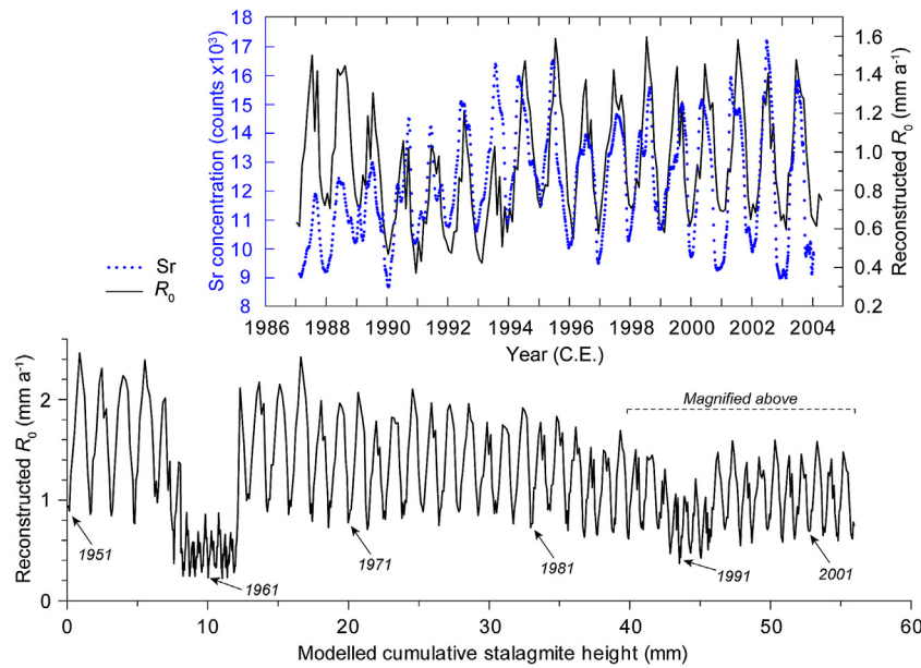
Fig. 6. The full R_0 reconstruction (black), with a magnification of the period January 1987 to April 2004 that is compared with Gib04a Sr concentration (blue). Sr data originally published by Mattey et al. (2008) . (For interpretation of the references to colour in this figure legend, the reader is referred to the web version of this article.)
