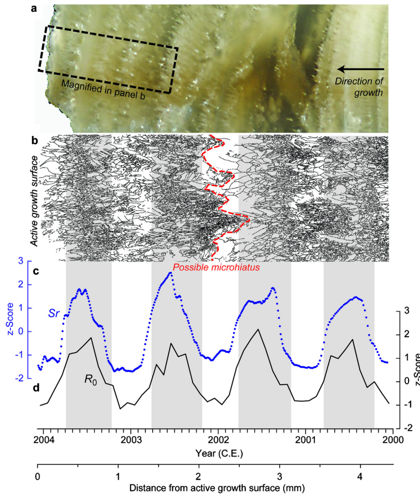
Fig. 7. Comparison of modelled growth during the period 2000 to April 2004 (corresponding to the upper \sim 4 mm of Gib04a) with (a) Gib04a petrography, (b) an electron backscatter grain boundary map of the area outlined in (a), and (c) high-resolution Sr concentration transect across the upper \sim 4 mm of Gib04a (blue), each of which were originally published by Matthey et al. (2010). (d) Reconstructed growth seasonality over this period, totalling 4.18 mm (black). Both Sr and R_0 are plotted as normalised z-scores, calculated by subtracting the mean and dividing by 1 standard deviation, so that the amplitude of seasonal changes in each dataset may be compared fairly. Vertical grey shading illustrates the association of R_0 , Sr, and grain-scale calcite fabric. See text for discussion. (For interpretation of the references to colour in this figure legend, the reader is referred to the web version of this article.)
