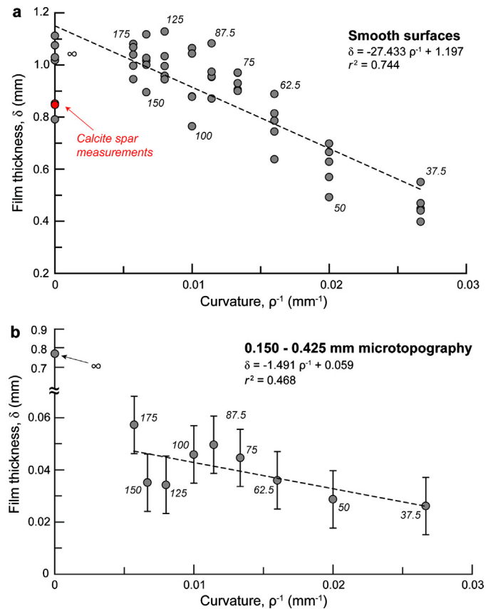
Fig. 4. Change in film thickness ( \delta ) as a function of surface curvature ( \rho ) for wetted surfaces; \delta increases with decreasing curvature. (a) Smooth surfaces ( r^2 = 0.74 ; p = 8.48 \times 10^{-16} ; n = 50 ) and (b) surfaces with 0.150 – 0.425 mm microtopography ( r^2 = 0.47 ; p = 0.09 ; n = 9 ). Mean values for wetted calcite spar (red; n = 7 ; \sigma = 0.012 ) are shown in (a). The \delta values determined for smooth surfaces are an order of magnitude greater than those for microtopographical surfaces. In the case of flat (infinite curvature) surfaces, \delta values are similar, indicating that wet Al provides a useful, though not perfect, analogue for calcite, supporting recent research (e.g., Collister and Matthey, 2008). (For interpretation of the references to colour in this figure legend, the reader is referred to the web version of this article.)
