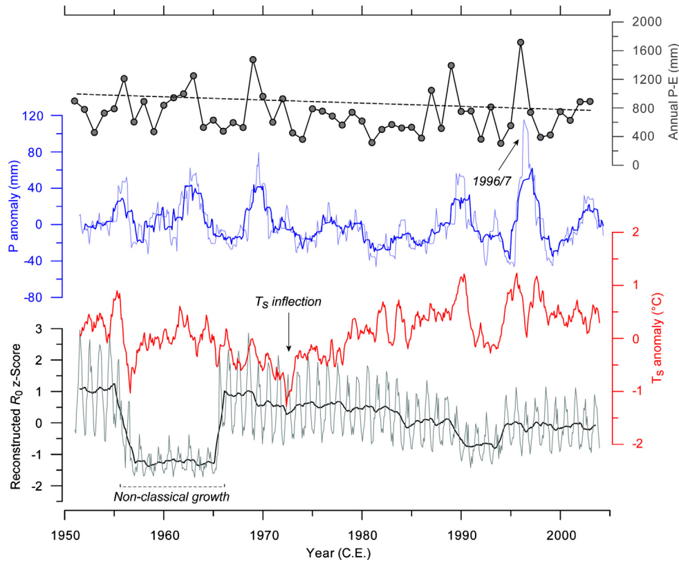
Fig. 8. Comparison of R_0 (grey; black curve is a 12-month running mean) with T_s anomalies (red), P anomalies (pale blue; dark blue curve is a 24-month running mean), and total annual water excess during the period 1951–2004 (grey). The non-uniform period of Gib04a growth (Fig. 6), an inflection in secular T_s variability, and the anomalously wet 1996/1997 winter are indicated. (For interpretation of the references to colour in this figure legend, the reader is referred to the web version of this article.)
