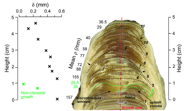
Fig. 5. Cut section of the modern growth of Gib04a (AD 1951–2004). The dotted line indicates the hiatus separating ancient (pre-Holocene) and modern growth, termed growth surface 1. The dashed lines indicate laminae 2 to 11. For each lamina, estimated curvature (mm) is given on the left, with corresponding mean \delta values plotted against height (see also Table 1). Laminae 2 and 3 (highlighted green) represent non-uniform stalagmite growth. The dashed red line indicates the vertical growth axis and the black arrows indicate clear inflections in laminae curvature that are visible in this 2-D cut section. See text for discussion. (For interpretation of the references to colour in this figure legend, the reader is referred to the web version of this article.)
