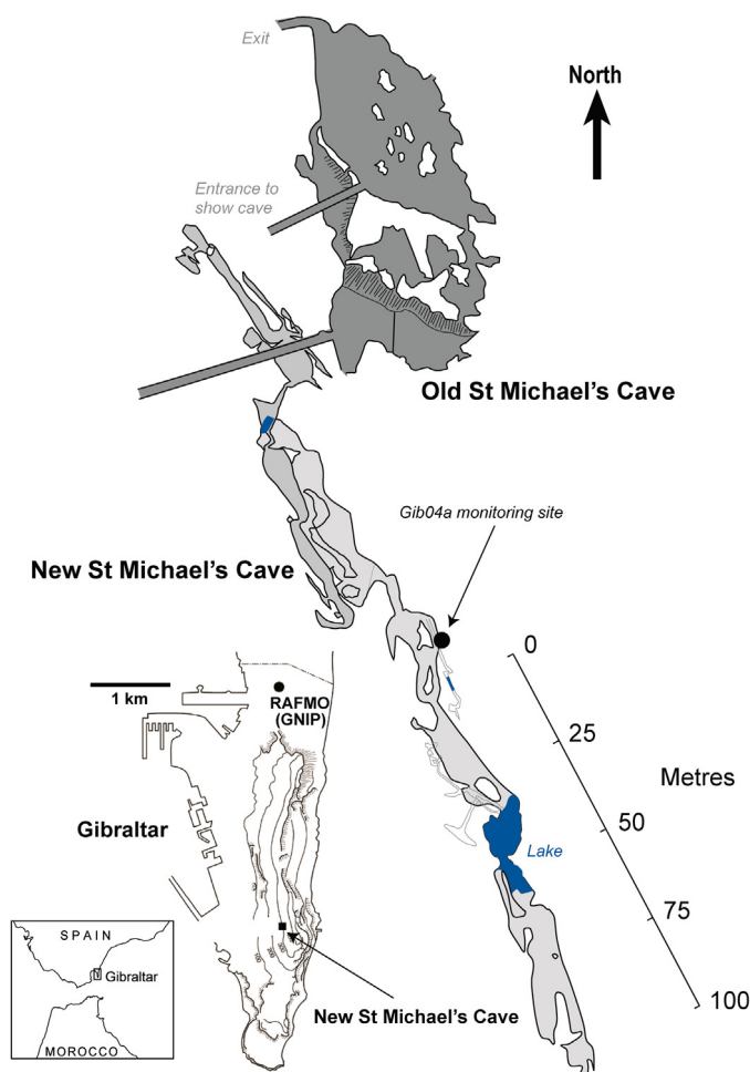
Fig. 1. Location and most recent survey map (undertaken in 2007) of NSM Cave and location and map of Gibraltar with locations of Gibraltar's RAFMO/GNIP station at North Front (World Meteorological Organisation station code: 8495; 36.2° N, 5.4° W, 5 m asl). Topographic contour lines on the Gibraltar map are in 100 metre intervals. Figure adapted from Matthey et al. (2010).
