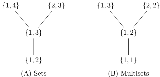
FIGURE 1. Part of the poset of (A) sets and (B) multisets under the majorization order.
