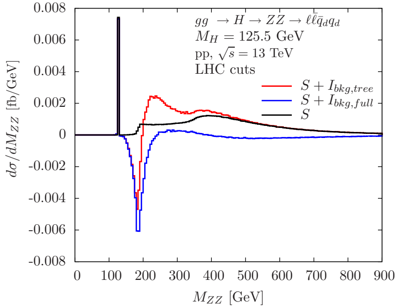
Figure 19. Invariant ZZ mass distributions for the signal process gg \rightarrow H \rightarrow ZZ \rightarrow \ell\bar{\ell}q\bar{d}q_d and including its interference with the background in pp collisions at \sqrt{s} = 13 \text{ TeV} . LHC cuts are applied (see main text). Other details as in figure 12.
