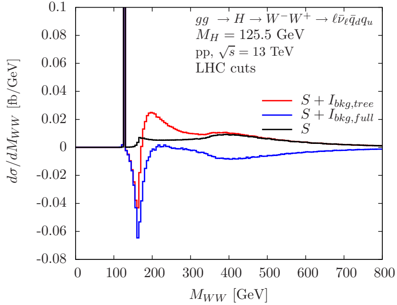
Figure 8. Invariant WW mass distributions for the signal process gg \rightarrow H \rightarrow W^- W^+ \rightarrow \ell \bar{\nu}_\ell \bar{q}_d q_u and including its interference with the background in pp collisions at \sqrt{s} = 13 \text{ TeV} . LHC cuts are applied (see main text). Other details as in figure 5.
