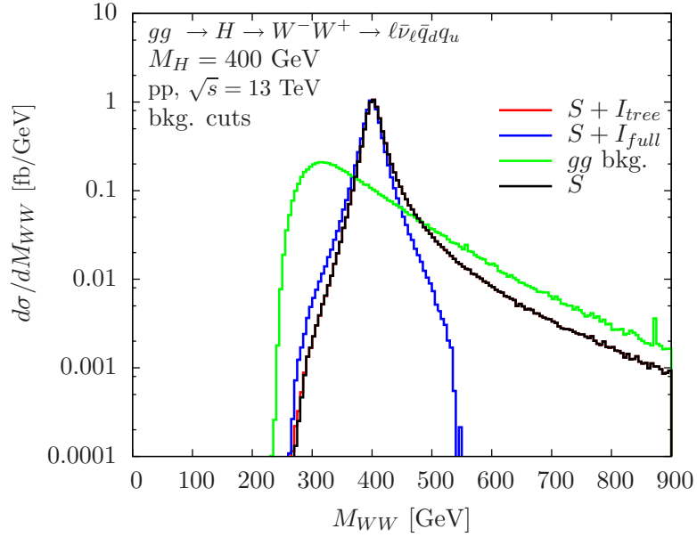
Figure 10. Invariant WW mass distributions for the signal process gg \rightarrow H \rightarrow W^-W^+ \rightarrow \ell\bar{\nu}_\ell q_u \bar{q}_d and including its interference with the background in pp collisions at \sqrt{s} = 13 TeV with background suppression cuts for a 400 GeV SM Higgs boson (see main text). Other details as in figure 9.
