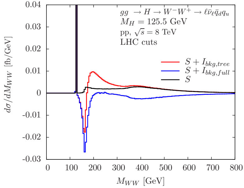
Figure 7. Invariant WW mass distributions for the signal process gg \rightarrow H \rightarrow W^- W^+ \rightarrow \ell \bar{\nu}_\ell \bar{q}_d q_u and including its interference with the background in pp collisions at \sqrt{s} = 8 \text{ TeV} . LHC cuts are applied (see main text). Other details as in figure 5.
