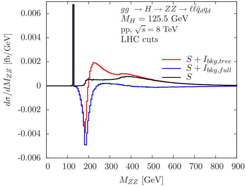
Figure 18. Invariant ZZ mass distributions for the signal process gg \rightarrow H \rightarrow ZZ \rightarrow \ell\bar{\ell}q\bar{d}q_d and including its interference with the background in pp collisions at \sqrt{s} = 8 \text{ TeV} . LHC cuts are applied (see main text). Other details as in figure 12.
