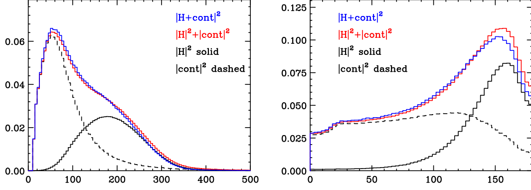
Figure 5: M_{l\bar{l}'} [GeV] (left) and \Delta\phi_{l\bar{l}'} [ ^\circ ] (right) distributions. Other details as in Fig. 3.
