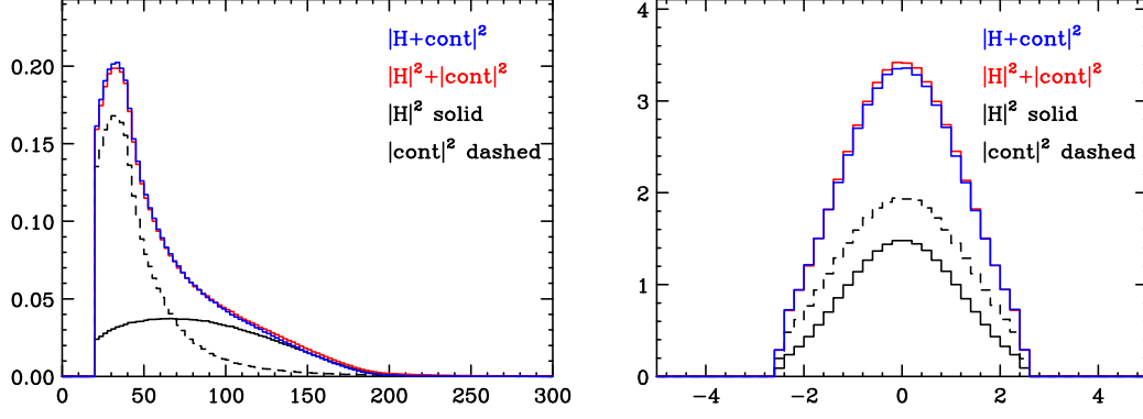
Figure 3: Differential cross section distributions for gg (\rightarrow H) \rightarrow W^-W^+ \rightarrow l\bar{\nu}_l\bar{l}\nu_l in pp collisions at \sqrt{s} = 7 TeV for M_H = 400 GeV and a single lepton flavour combination calculated at LO. The p_{Tl} [GeV] (left) and \eta_l (right) distributions are shown. Standard cuts are applied (see main text). fb is used as cross section unit.
